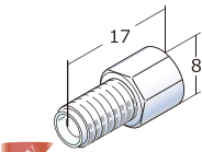
NEW Name: 1/8" HEX Flat seal Fittings P/N: 9822D Material: ETFE Quantity: 10 / pack
