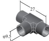
Name: T-joint P/N: 9121 Material: PEEK Thread: M8×1 ID: 1.0 mm Quantity: 1
