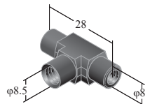
Name: Reducing T-joint P/N: 9108 Material: PEEK Thread: No.10-32, 1/4-28UNF ID: 1.0 mm Quantity: 1
