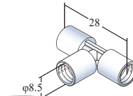
NEW Name: T joint P/N: 9825D Material: ETFE Thread: 1/4-28UNF ID: 1.0 mm Quantity: 1
