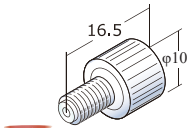
NEW Name: 1/16" Fittings D P/N: 9820D Material: ETFE Quantity: 10 / pack
