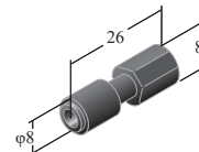
Name: Reducing Union P/N: 9112 Material: PEEK Thread: No.10-32UNF, Syringe ID: 1.0 mm Quantity: 1
