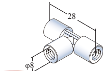
NEW Name: T-joint P/N: 9824D Material: ETFE Thread: No.10-32UNF ID: 1.0 mm Quantity: 1
