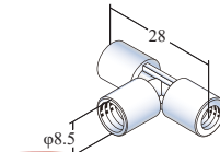
NEW Name: Reducing T-joint P/N: 9826D Material: ETFE Threads: No.10-32UNF, 1/4-28UNF ID: 1.0 mm Quantity: 1
