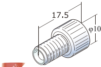
NEW Name: 1/8" Flat seal Fittings P/N: 9823D Material: ETFE Quantity: 10 / pack
