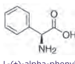
L-(+)-alpha-phenylglycine
