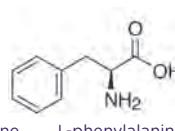
L-phenylalanine
